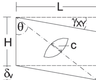
Fig. 3. Diagonal crack (c) because of differential settlement ( \delta_v )
